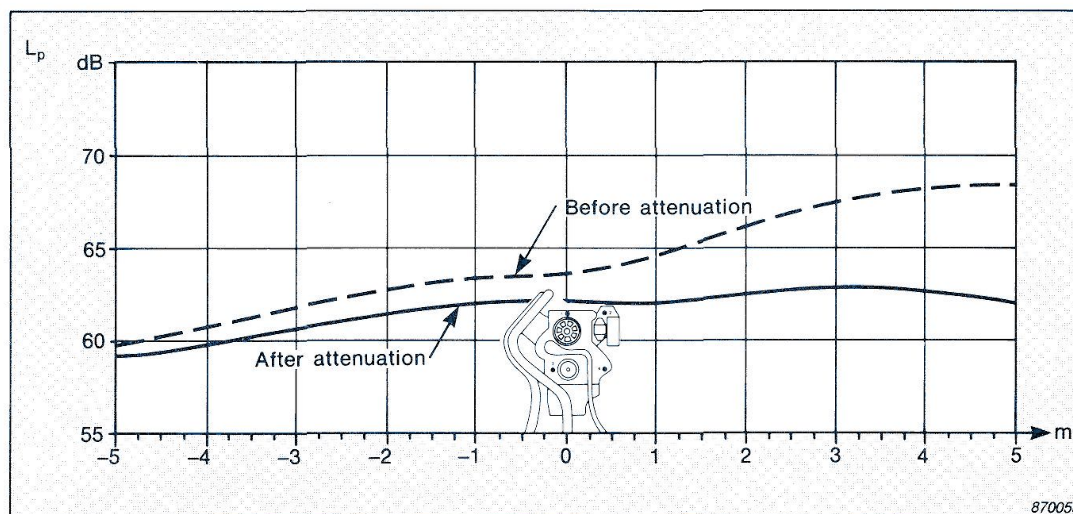
Fig. 16. Sound Pressure Level along a line at 7.5\text{m} distance, 1\text{m} above a non-reflective ground, before and after attenuation of the right cylinder bank. The results are for the 400\text{Hz} 1/3 -octave band
