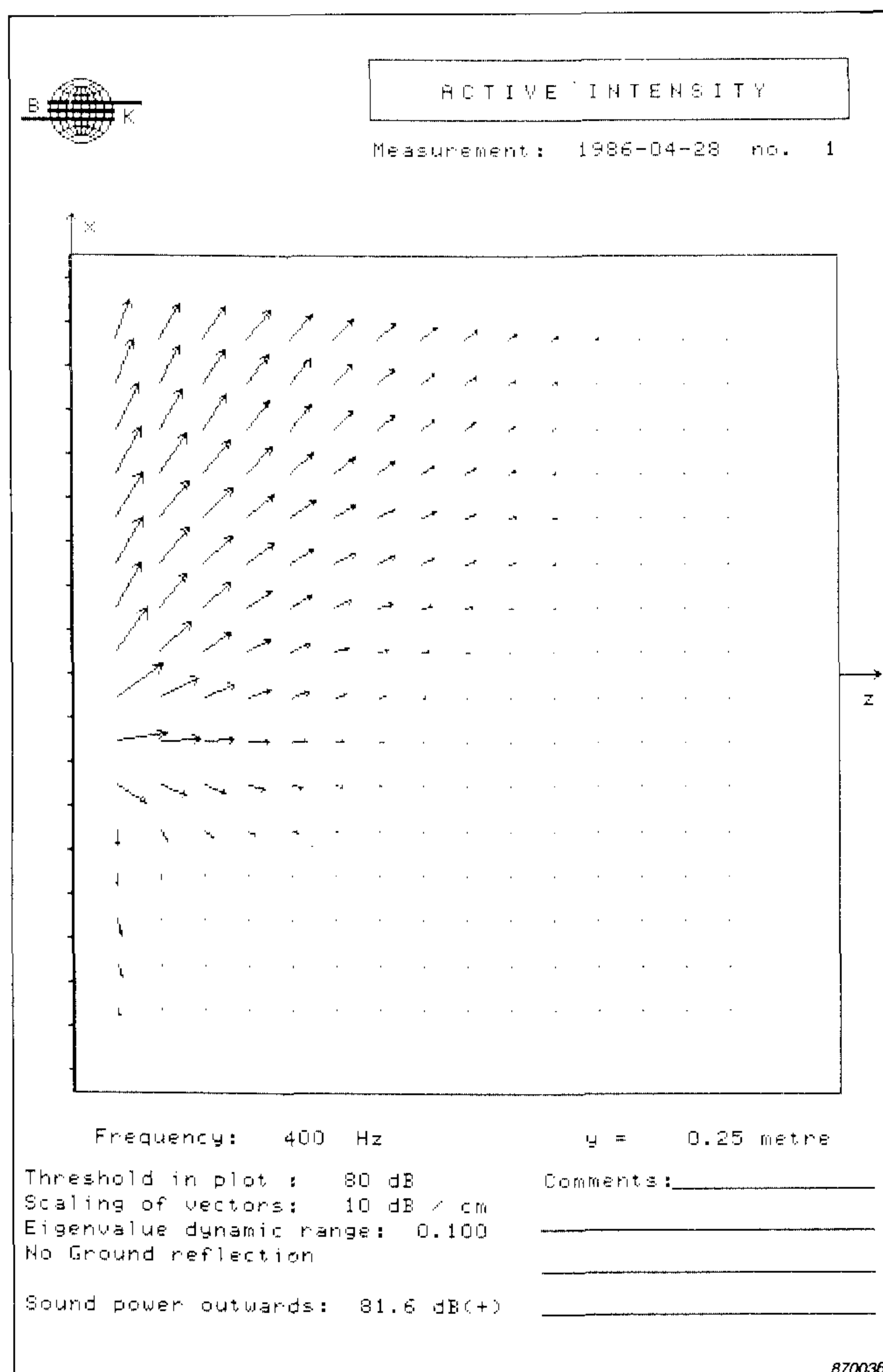
Fig. 10. Plots of intensity vectors in the plane y = 0,25 m for the 400 Hz 1/3 -octave band. a) Active intensity b) Reactive intensity
