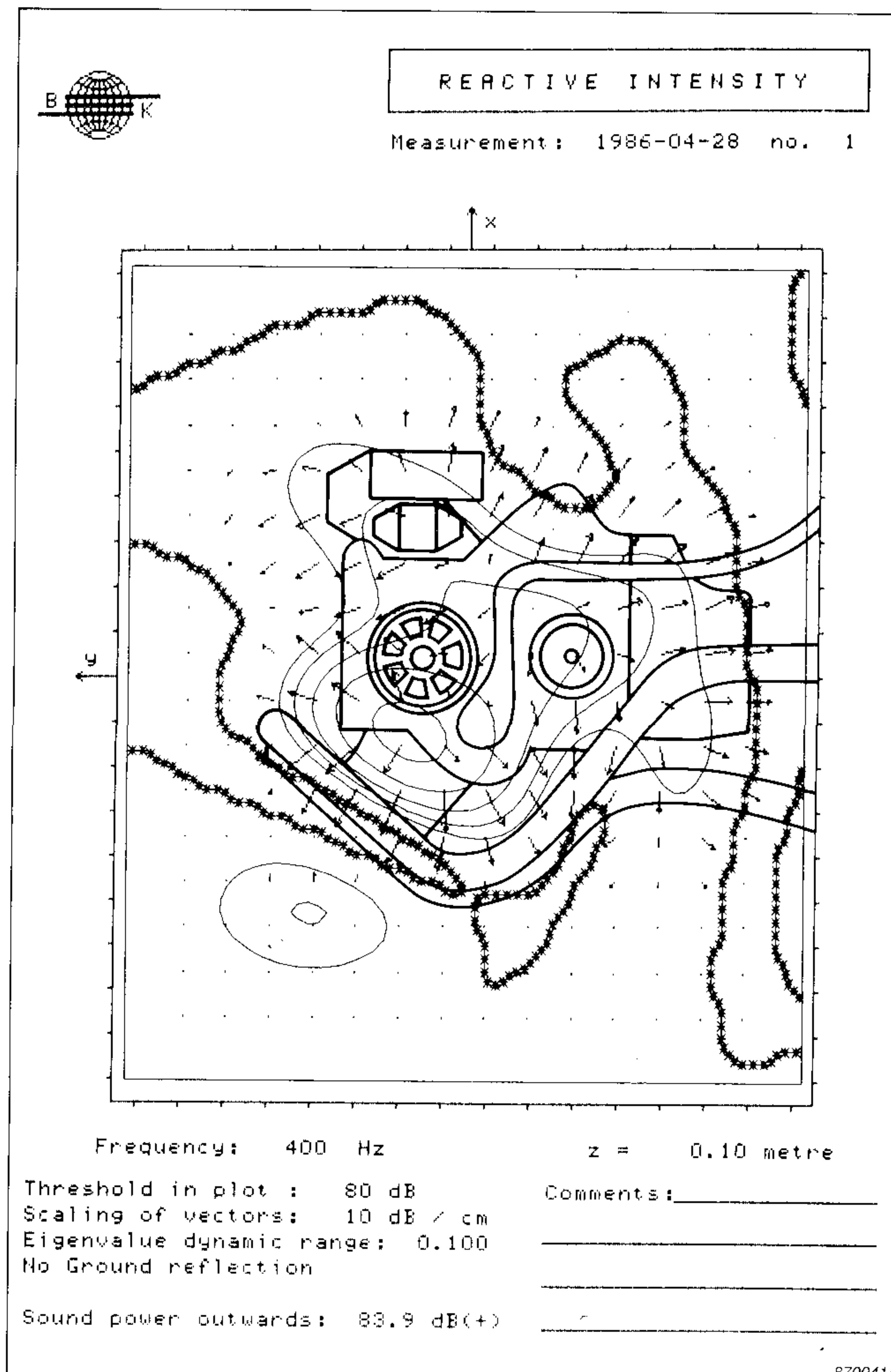
Fig. 12. Combined contour/vector plots of intensity in the plane z = 0,1 m for the 400 Hz 1/3 -octave band
