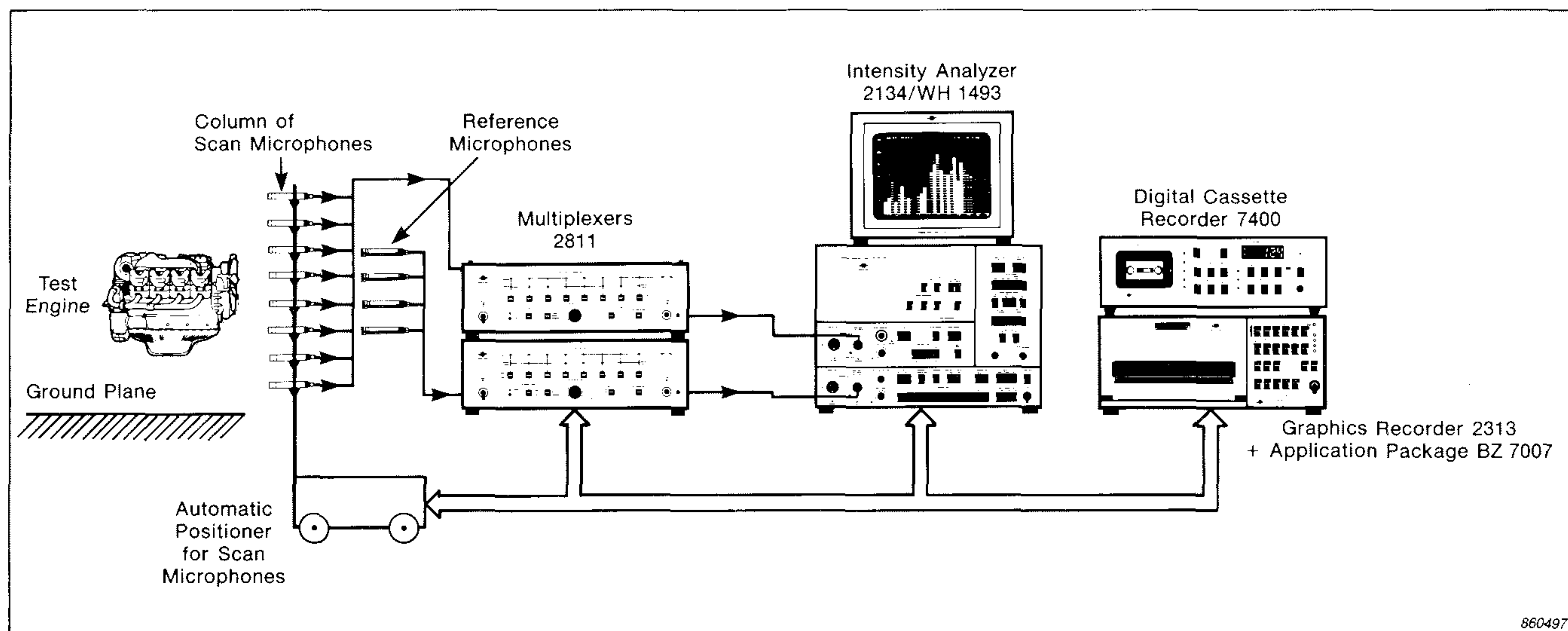
Fig. 1. Instrumentation for STSF
