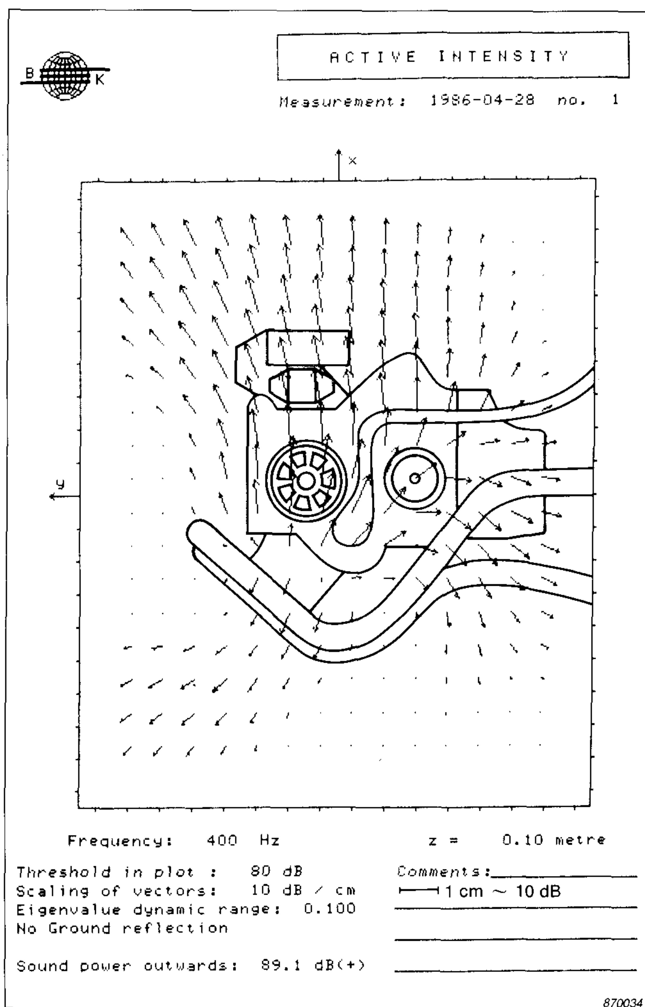
Fig. 9. Plots of intensity vectors in the plane z = 0,1 m for the 400 Hz 1/3 -octave band produced by 2313/BZ 7007
