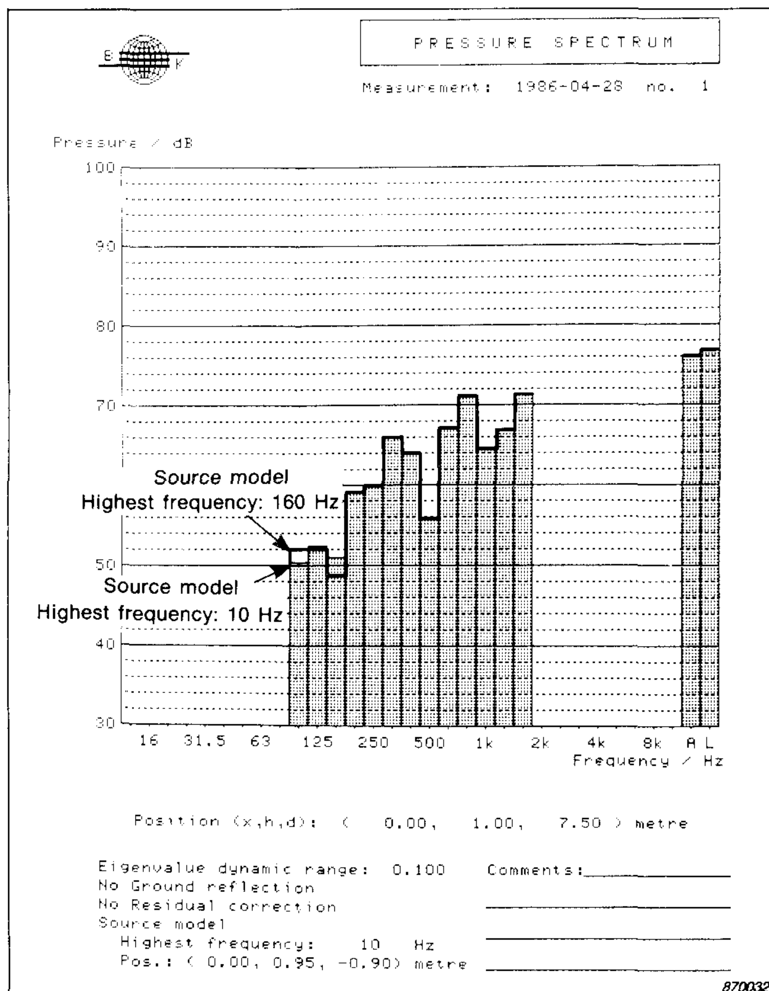
Fig. 7. Sound pressure level at 7,5m distance, 1m above ground, with and without source model for frequencies up to 160 Hz
