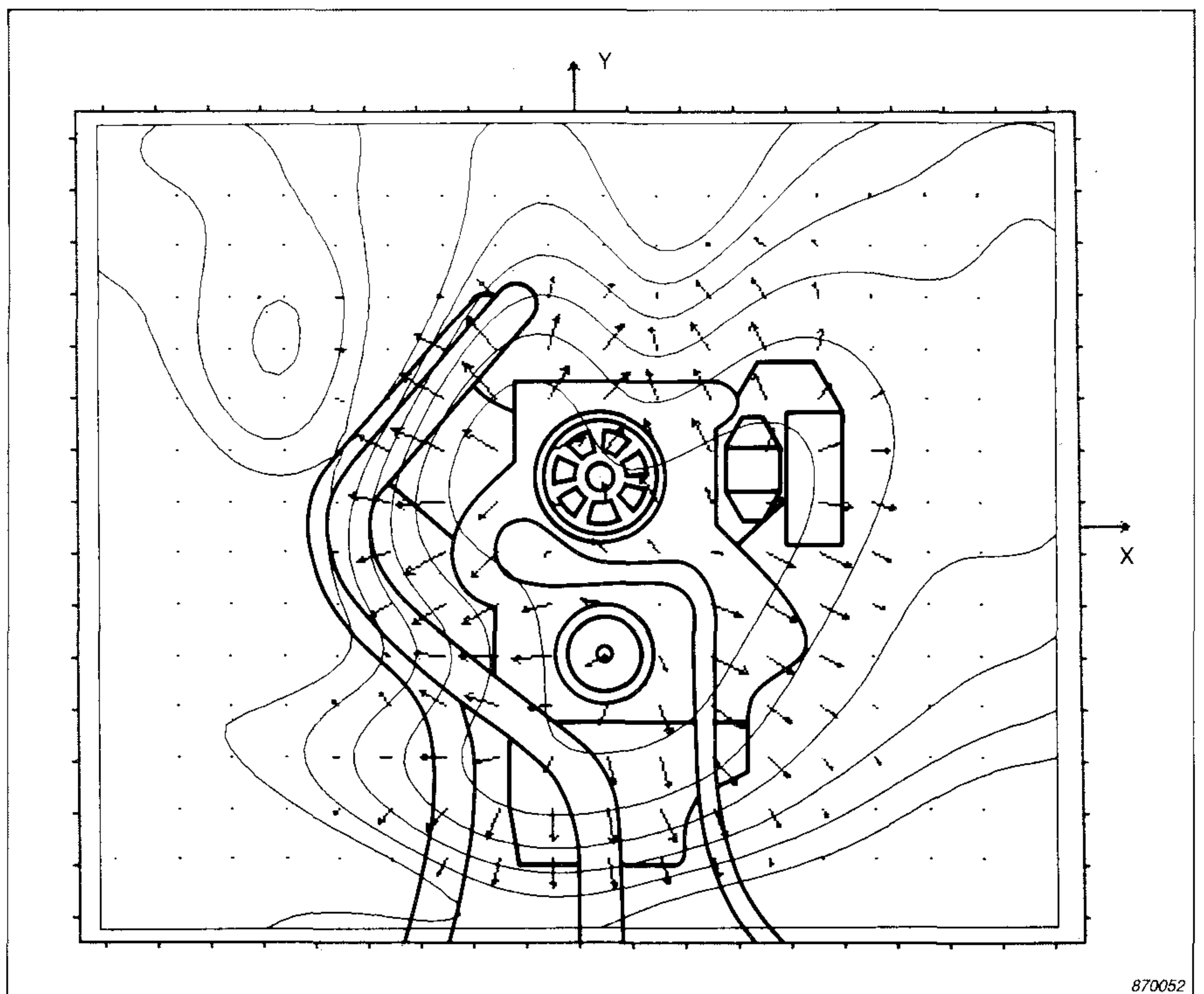
Fig. 13. Combined pressure contour/reactive vector intensity plot in the plane z = 0,1\text{m} for the 400 Hz 1/3 -octave band. The threshold level is 80 dB and the contour interval is 2 dB
