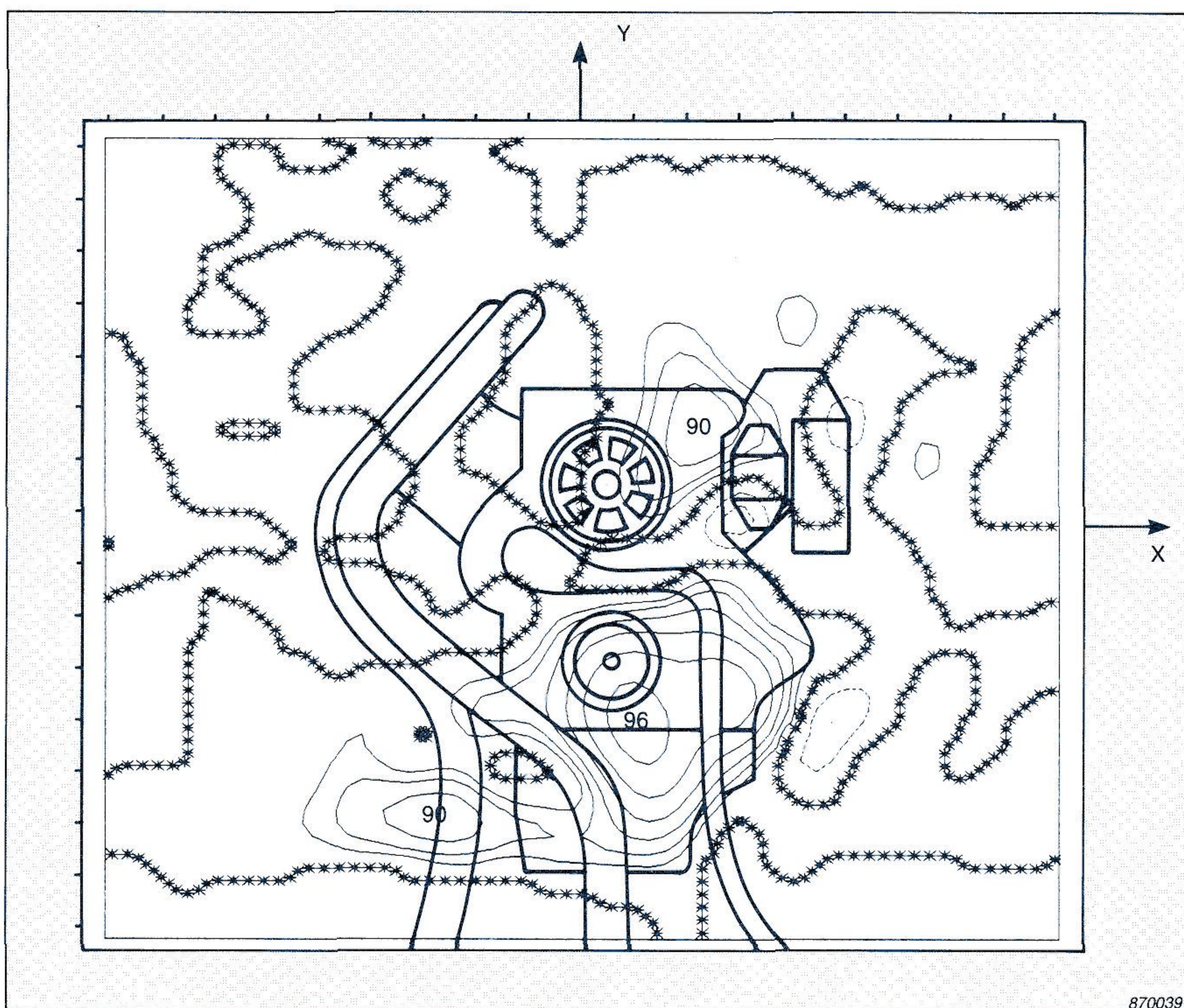
Fig. 15. Contour plot of active intensity in the plane z = -0.2\text{m} for the 400\text{Hz} 1/3 -octave band after attenuation of the right cylinder bank. The threshold level is 84\text{dB} and the contour interval is 2\text{dB}
