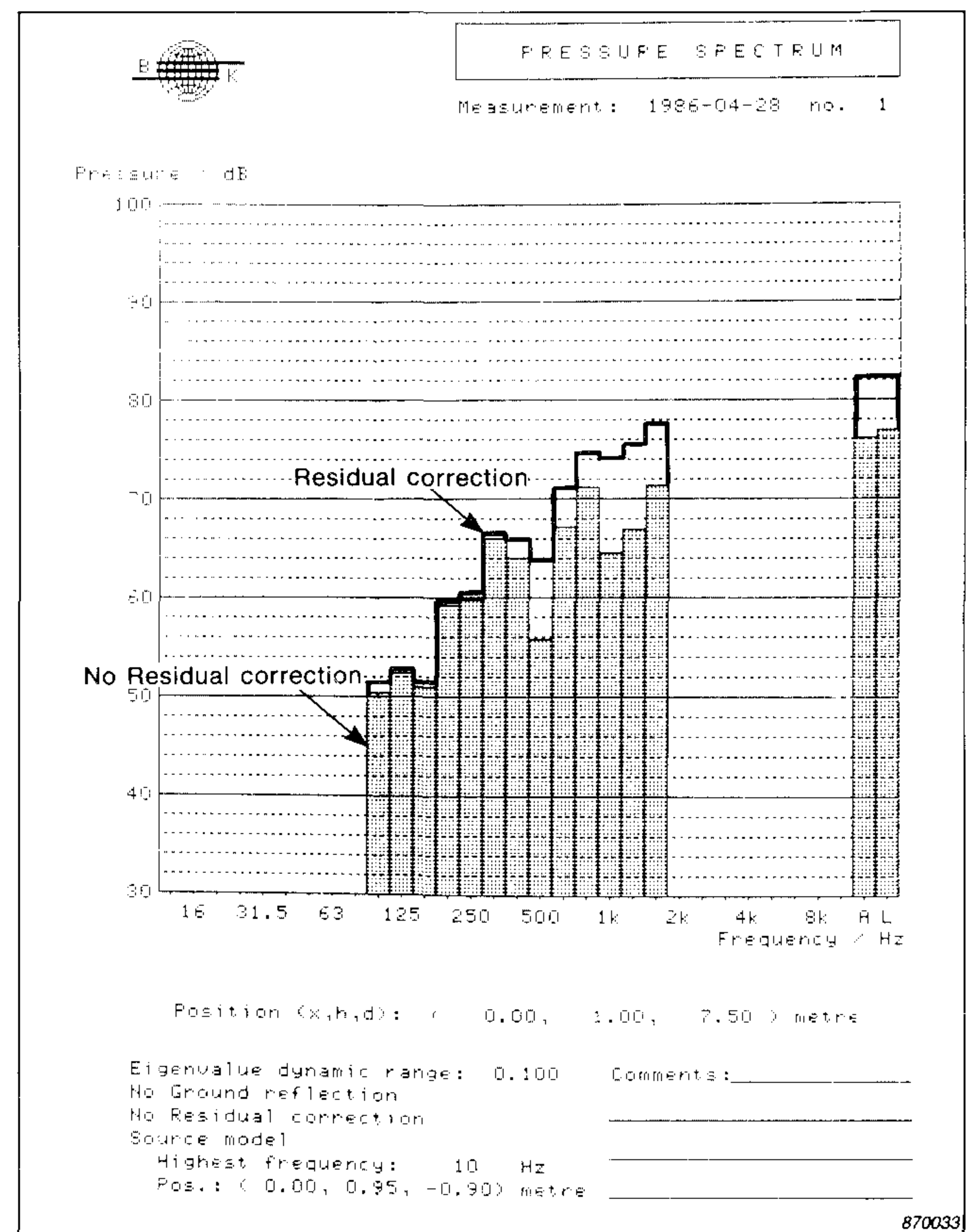
Fig. 8. Sound pressure level spectrum at 7,5m distance, 1m above ground, with and without residual correction
