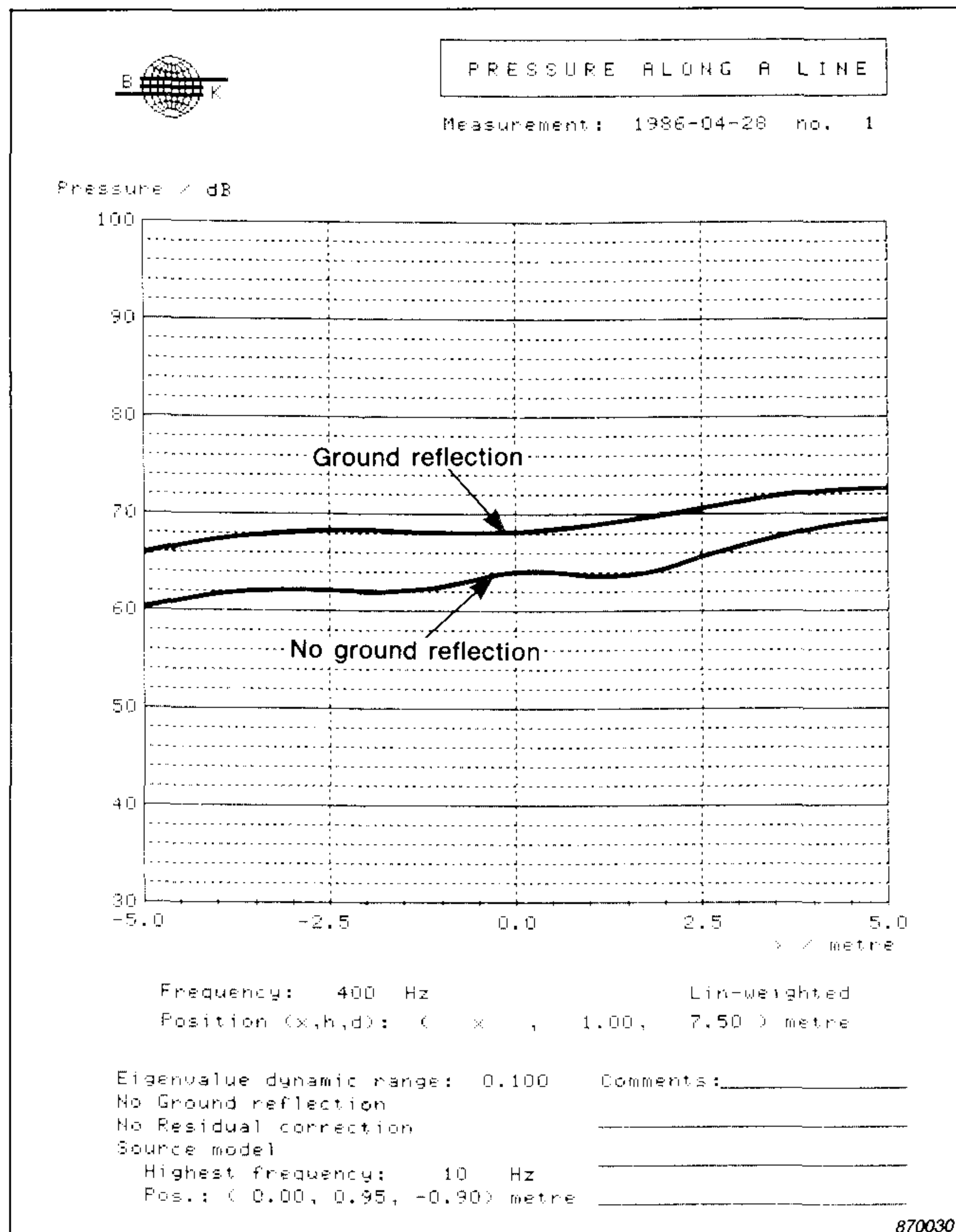
Fig. 5. Sound pressure level at 7,5m distance with and without a reflecting ground plane for the 1/3 -octave band at 400 Hz
