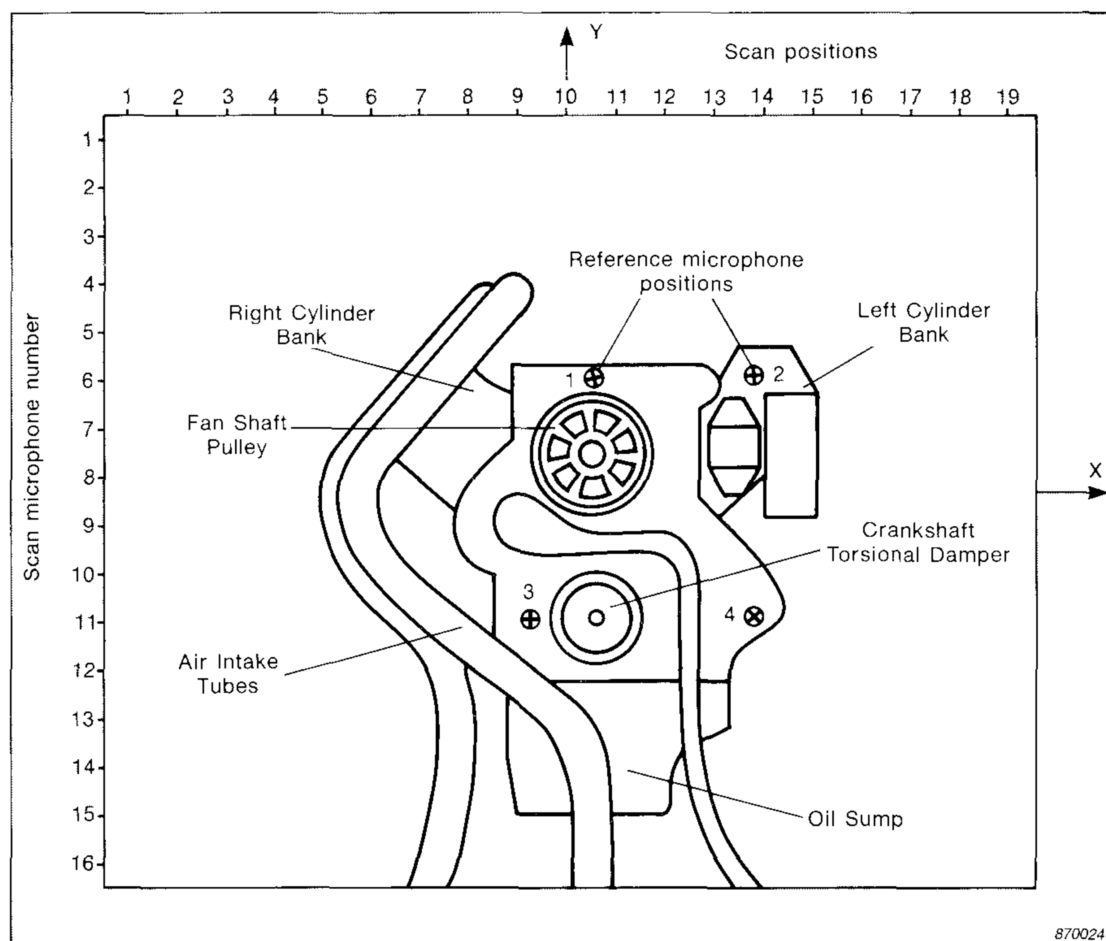
Fig. 2. Position of the 4 reference microphones the measurement positions and the outline of the 8 cylinder diesel supercharge 14 litre engine seen in the xy plane
