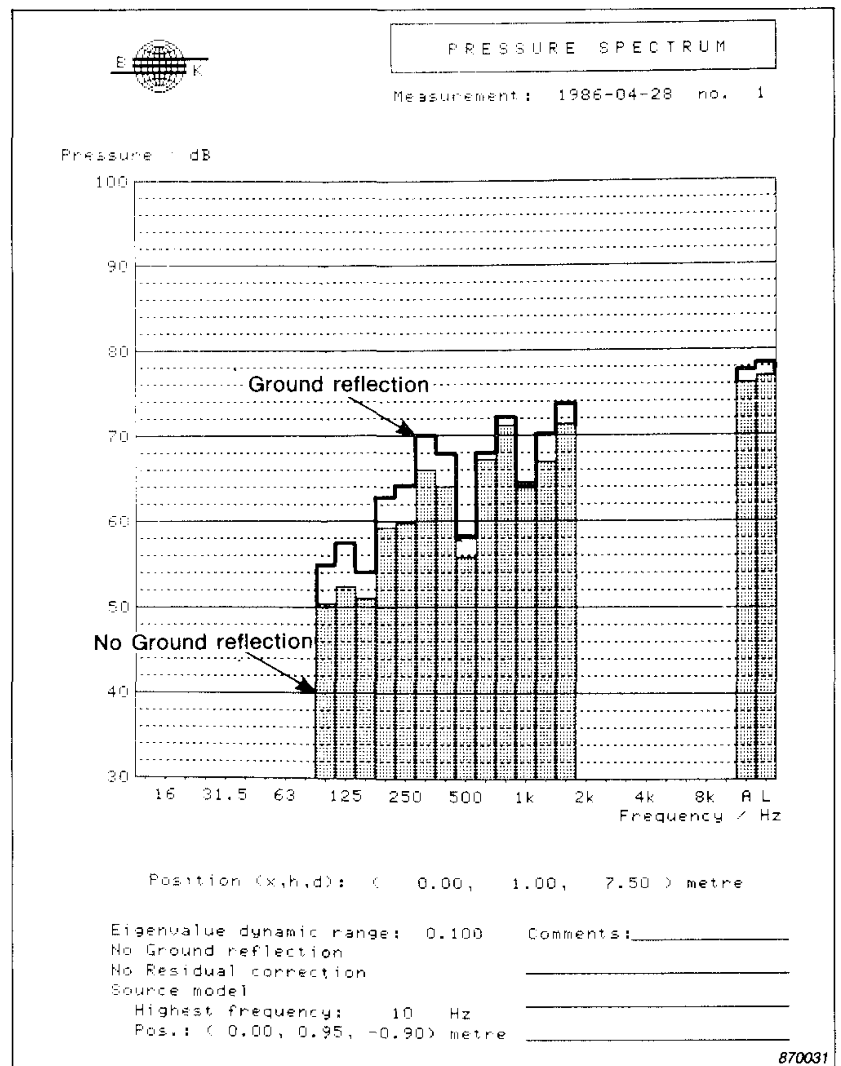
Fig. 6. Sound pressure level spectrum at 7,5m distance, 1m above ground, with and without reflective ground
